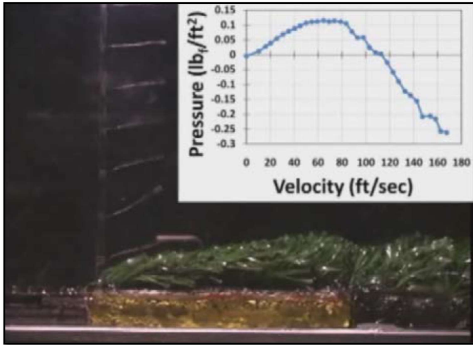
Figure 5. ClosureTurf® Lift and Drag Testing at GTRI
