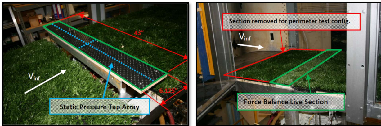
Figure 4. ClosureTurf® GTRI Test Configuration
