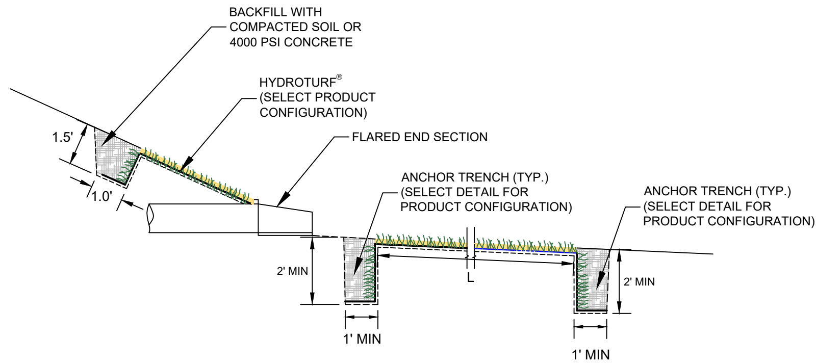
B HYDROTURF® OUTFALL PIPE 1 PROFILE NTS
