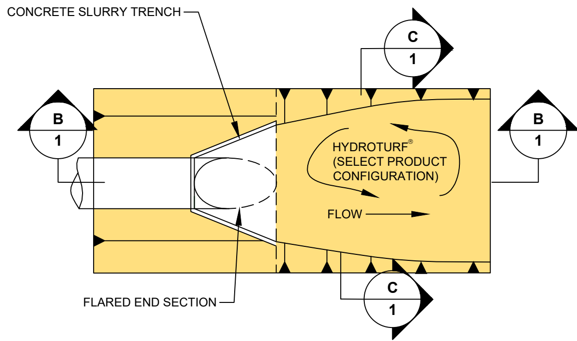
A HYDROTURF® AT OUTFALL PIPE 1 PLAN NTS
