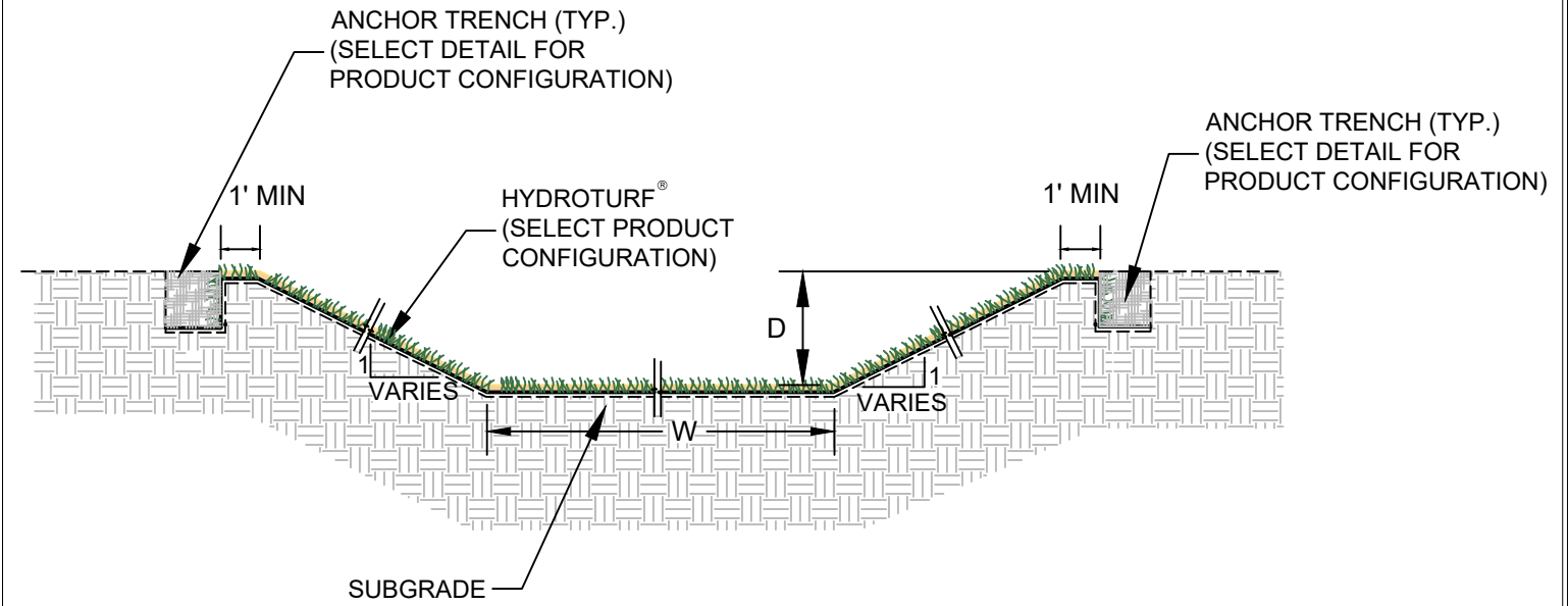
C HYDROTURF® OUTFALL PIPE 1 SECTION NTS
