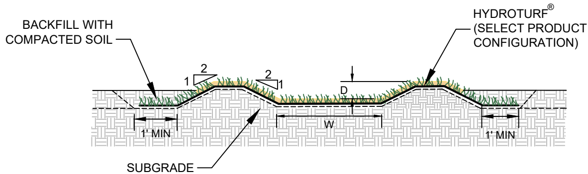
A 2 OPTION 2 DOWNSLOPE CHANNEL SECTION
